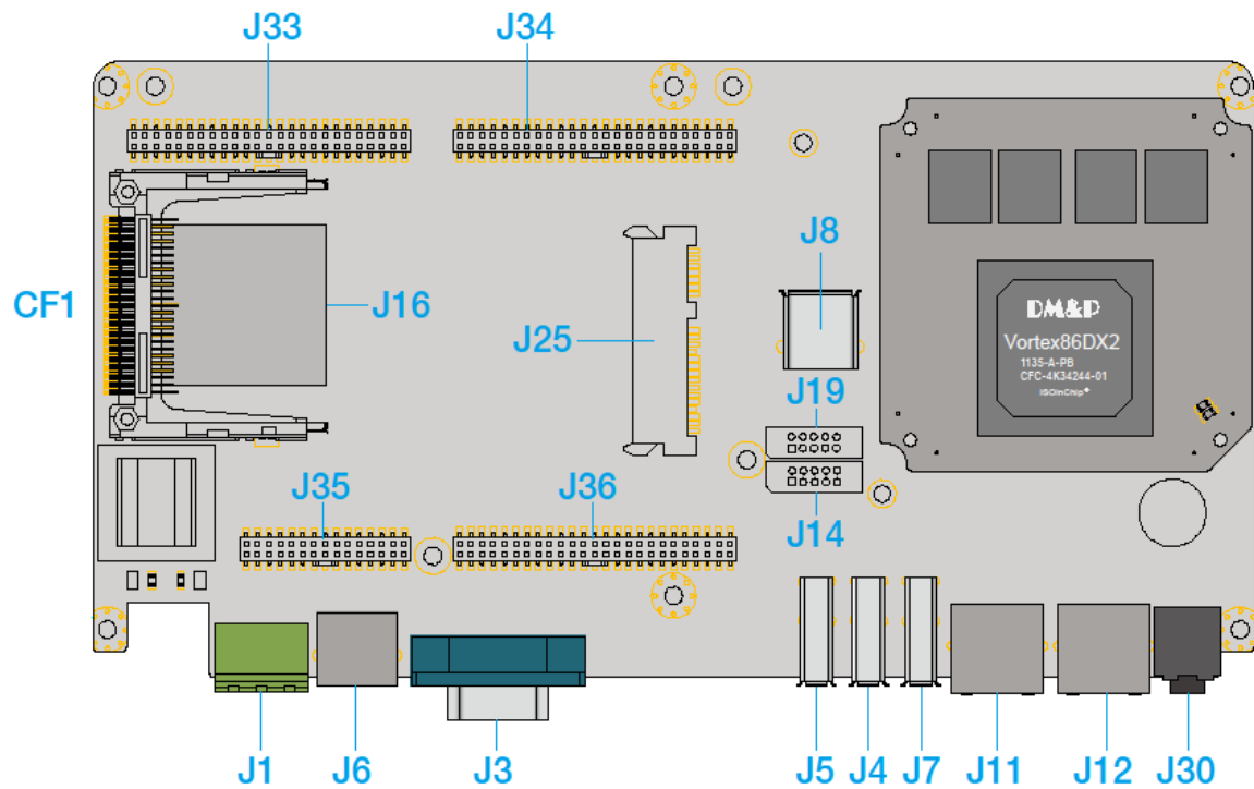
PPC CPU Board
